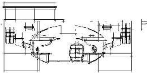
CROSS SECTION 2 - TRAIN PLATFORM 1:200 SCALE
